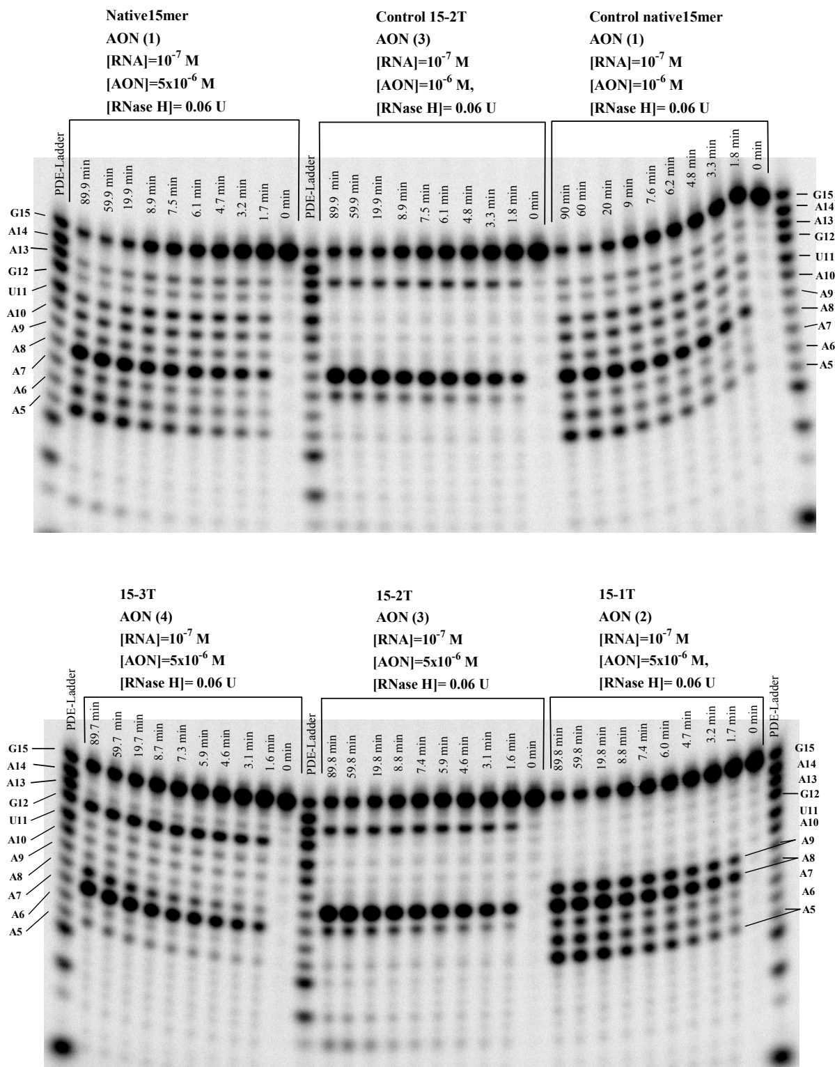
Figure S6. Autoradiograms of 20% denaturing PAGE, showing the cleavage kinetics of 5'- ^{32} P-labelled target RNA ( 14 ) by RNase H1 in the native AON ( 1 )/RNA ( 14 ) and single, double and triple oxetane T modified AON ( 2-4 )/RNA ( 14 ) hybrid duplexes. The kinetics of the control native 15mer AON ( 1 ) and double T AON ( 3 ) with 1 \mu M and RNA ( 14 ) with 0.1 \mu M concentration, used for the calibration of the exact RNase H concentration, are also shown. PDE-Ladder: snake venom PDE ladder. Conditions of cleavage reaction: RNA (0.1 \mu M) and AONs (1 or 5 \mu M) in buffer, containing 20 mM Tris-HCl (pH 8.0), 20 mM KCl, 10 mM MgCl 2 and 0.1 mM DTT at 21 °C, 0.06 U of RNase H. Total reaction volume is 30 \mu l. (See Materials and Methods section for full experimental details.)
